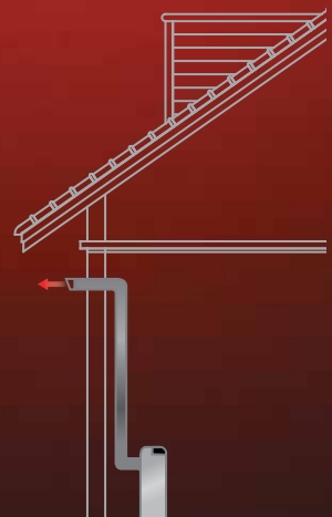
Through-Wall Vent Termination with Extension Kit and Elbow
